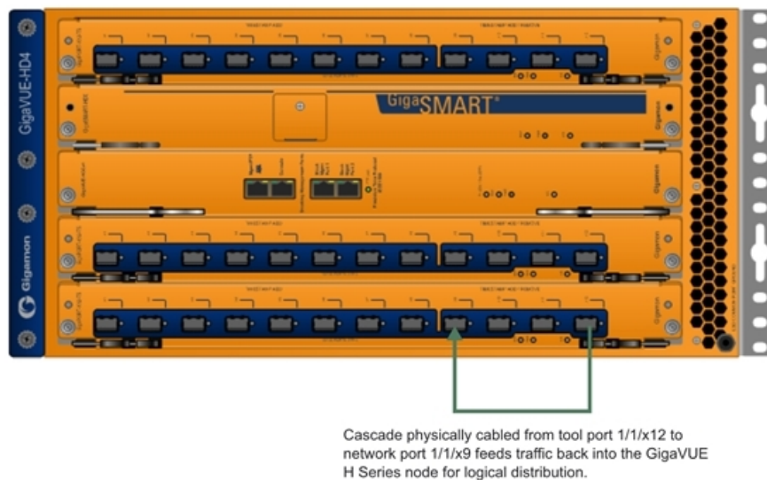
Figure 151 Cascade Physically Cabled from Tool to Network Port
