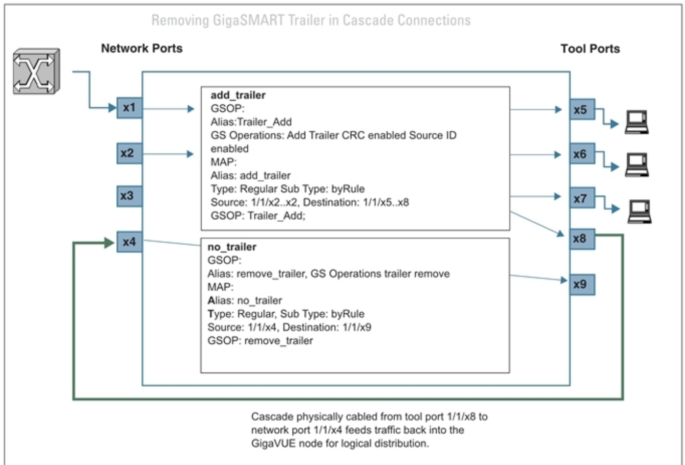
Figure 152 Removing the GigaSMART Trailer from a Cascade Connection
