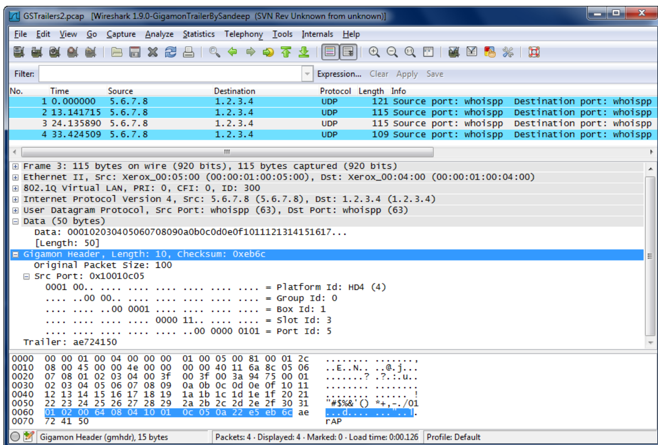
Figure 154 Wireshark Decode of GigaSMART Trailer
