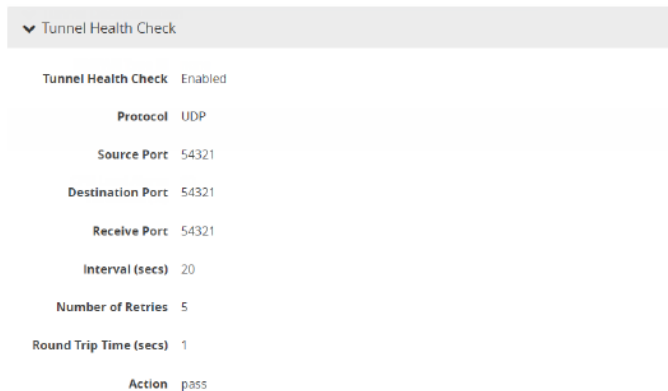
Figure 138 Configure UDP Health Check Parameters
