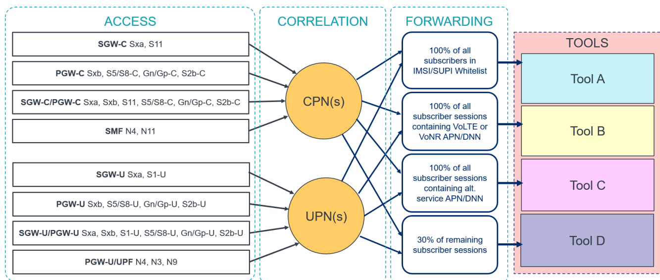
Figure 23 CUPS Traffic Visibility Solution
